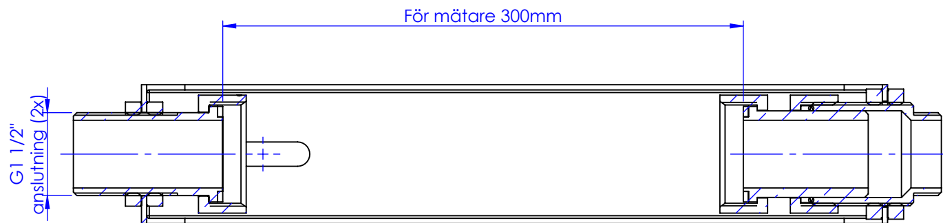
SECTION B-B
